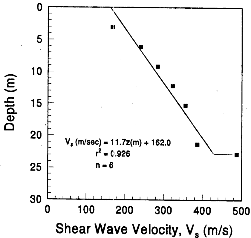
Figure 3-12. Shear Wave Velocity Profile from SASW Survey.
