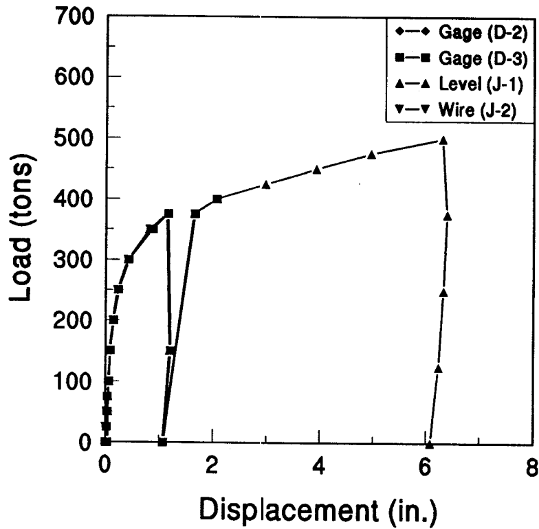
Figure 5-2. Full Range of Axial Load-Displacement Response for Floating Shaft C2.
